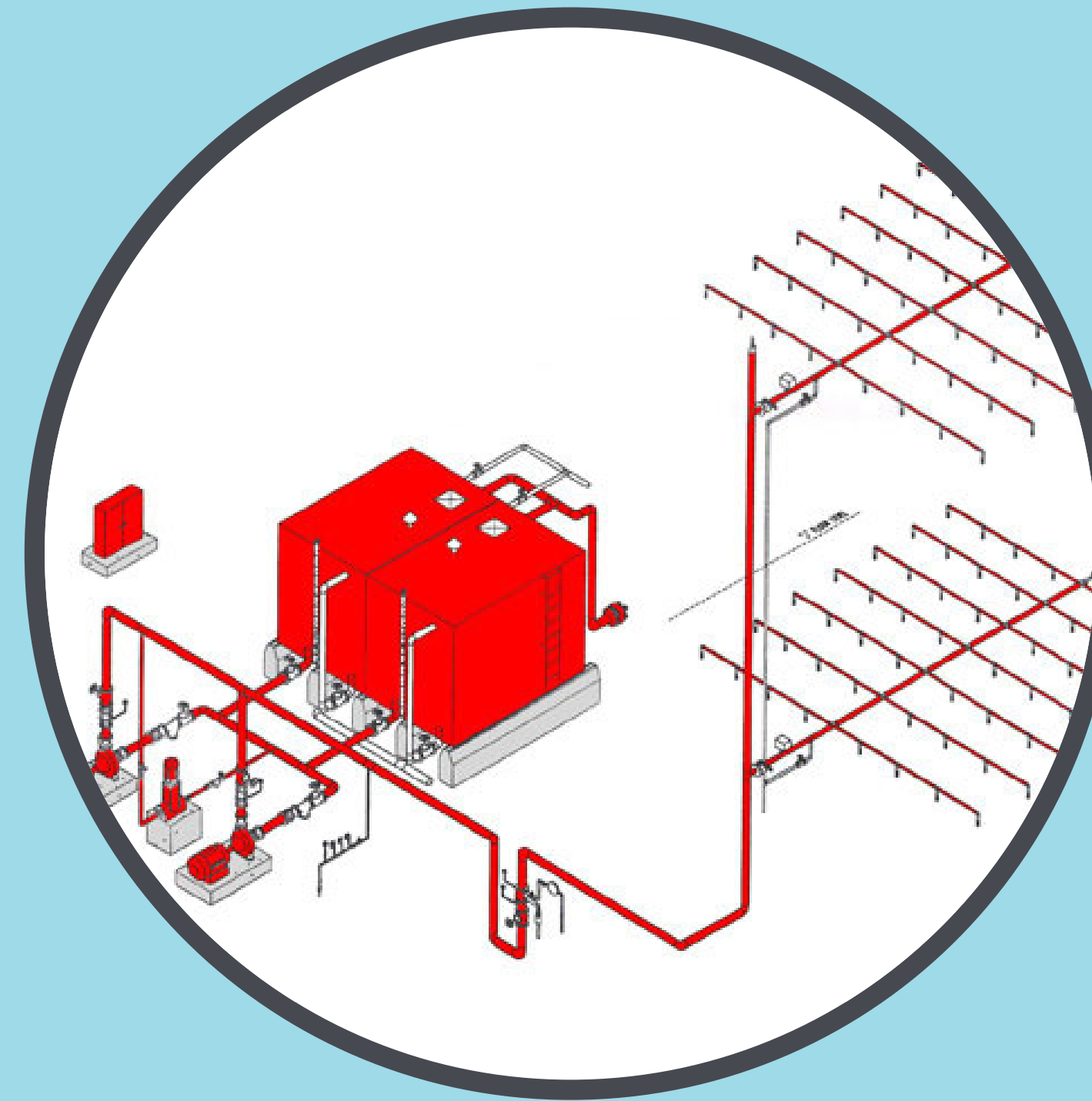
FOAM SYSTEM
